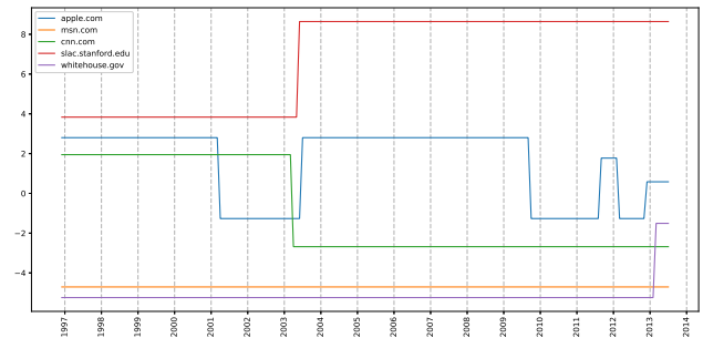
(b) Sudden moves of similarity, as identified by an HMM
