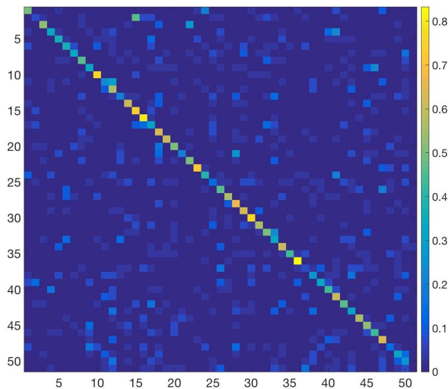
Figure 5. Confusion matrix on the HMDB51 dataset using our best model. The x-axis denotes the predicted labels and the y-axis represents the ground truth labels for 51 action classes.
