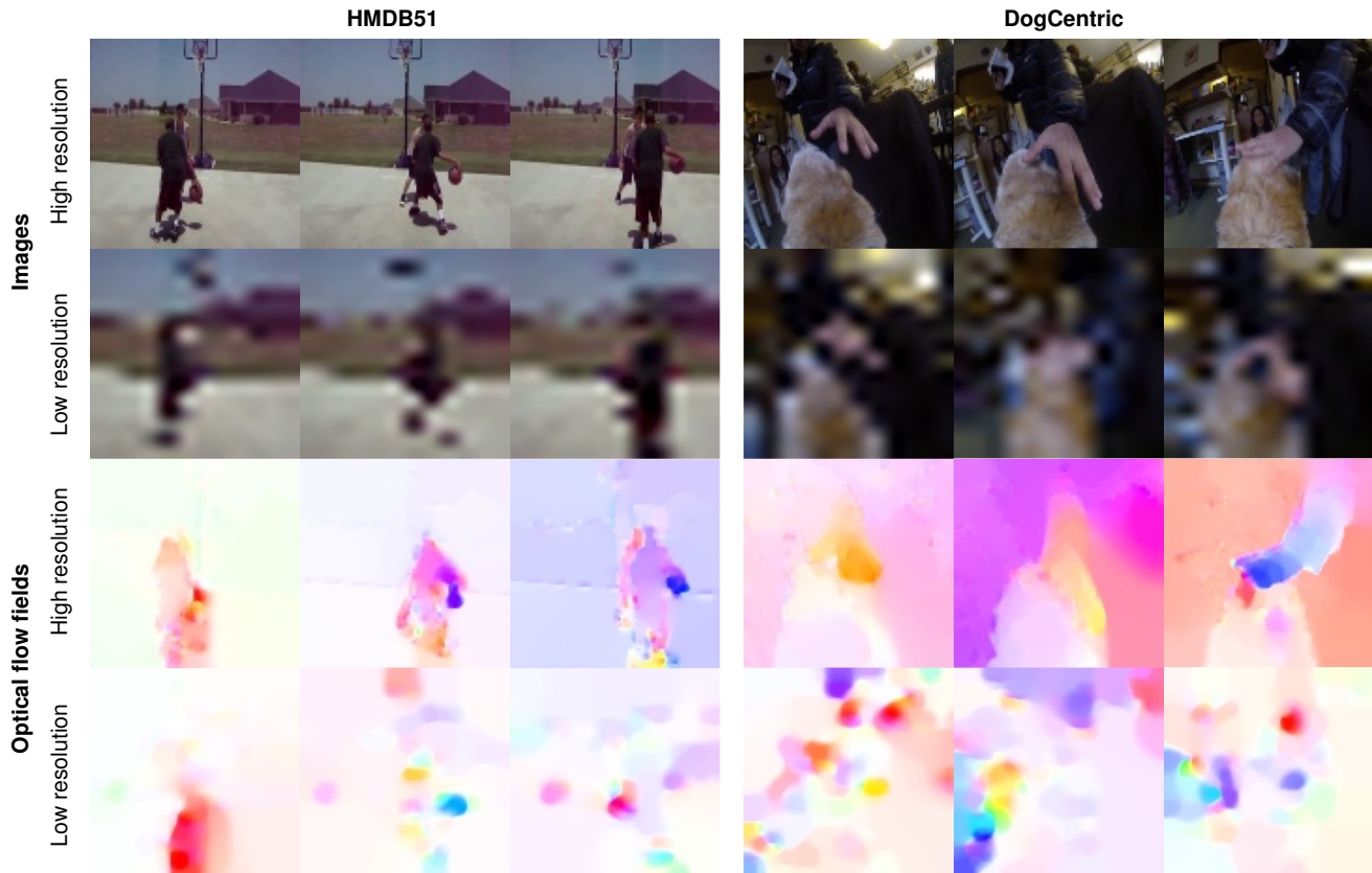
Figure 4. Examples of video frames from the HMDB51 (left) and DogCentric (right) datasets. First row : high resolution images resized to 112 \times 112 pixels; Second row : low resolution ( 12 \times 16 pixel) images upsampled to 112 \times 112 with bi-cubic interpolation; Third and fourth rows : optical flow fields for high resolution and low resolution images, respectively, calculated from images rescaled to 112 \times 112 .
