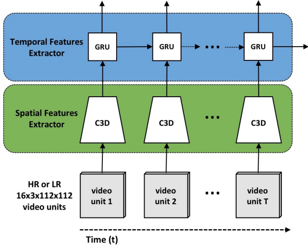
Figure 2. Visualization of our spatiotemporal features extractor, which uses a C3D network to capture spatial and temporal features for video units and an RNN to encode motion information across the entire video stream.
