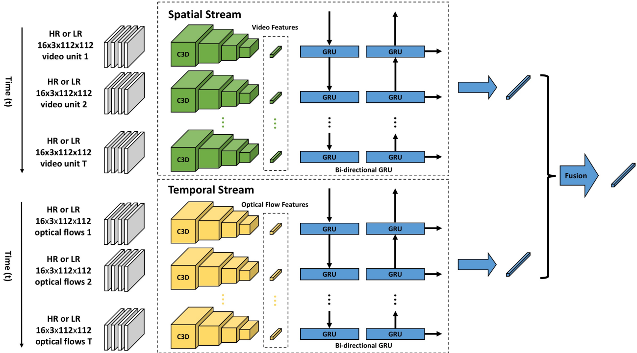
Figure 3. Visualization of our fully-coupled two-stream spatiotemporal networks. We feed RGB frames into the spatial stream (green) and corresponding stacked optical flow fields to the temporal stream (yellow). The GRU networks (blue) compute spatiotemporal information for the entire video using the extracted C3D features as inputs. In training, both C3D and GRU are fully-coupled with convolution filters shared between high and low resolution training videos, whereas only low resolution videos are used in testing.
