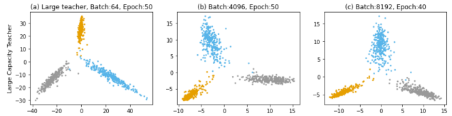
Figure 7: Improved penultimate layer representation for large capacity teach on MNIST. (a) shows the tight clusters, (b) and (c) shows similar clustering for different batch sizes and number of epochs.
