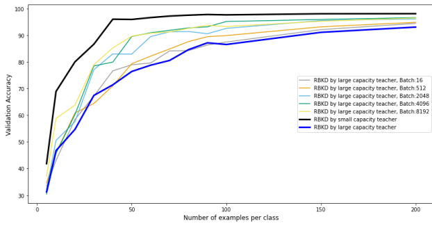
Figure 8: Improved number of examples required per class for distillation on MNIST
