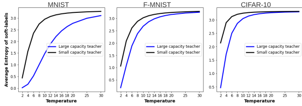
Figure 3: Average entropy of teacher’s response for MNIST, Fashion-MNIST and CIFAR-10 datasets.
