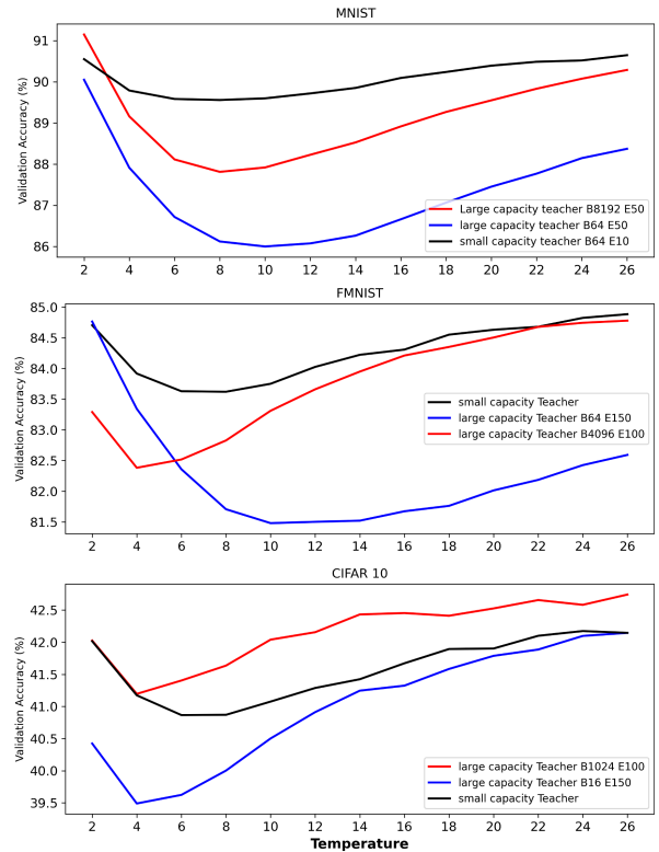
Figure 9: Improved performance on training with suitable batch size and epochs,
