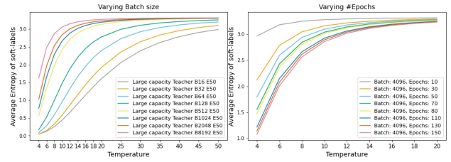
Figure 6: Variation in average entropy of soft-label vs temperature. Left, for different batch sizes at epoch 50. Right, for different epochs at batch size 4096 on MNIST dataset.
