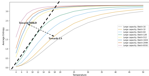
Figure 10: The distillation hypothesis in terms of average entropy of soft-labels.
