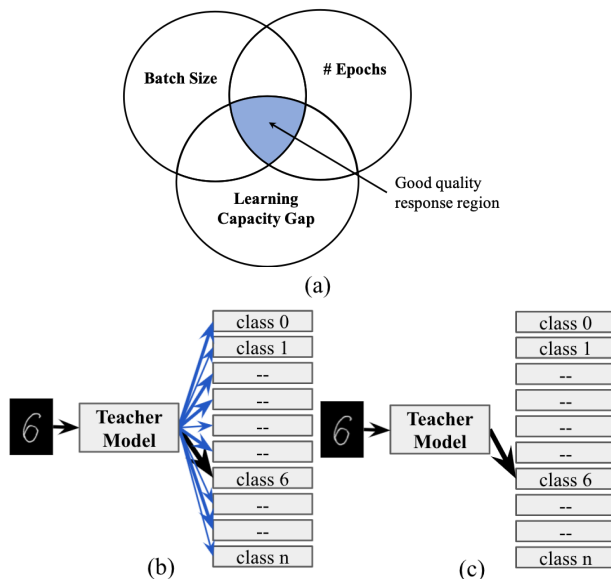
Figure 1: (a) Sweet spot between batch size and number of epochs for a given teacher-student pair for effective KD. (b) and (c) Difference in teacher’s response in presence and absence of similarity information, respectively.
