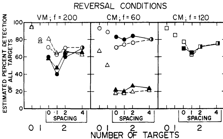
Figure 4. Data from Experiment 2. Probabilities of correctly detecting one target when one was presented, or two targets when two were presented, as a function of spacing, for each condition. The data shown have been adjusted to remove effects of guessing and false alarms. The observed percentage of "none" responses to no-target trials is also shown. Circles show the estimated percentage of detection prior to reversal (data from Experiment 3, Part I), while triangles indicate performance after reversal in Experiment 2. The squares in the right-hand panel show post-reversal detection from Experiment 2 after frame time was increased to 120 msec. The open symbols and dashed lines indicate the II conditions (identical targets); the closed circles and solid lines indicate the NI conditions (different targets). (VM = varied mapping; CM = consistent mapping; f = frame time, in msec.)
