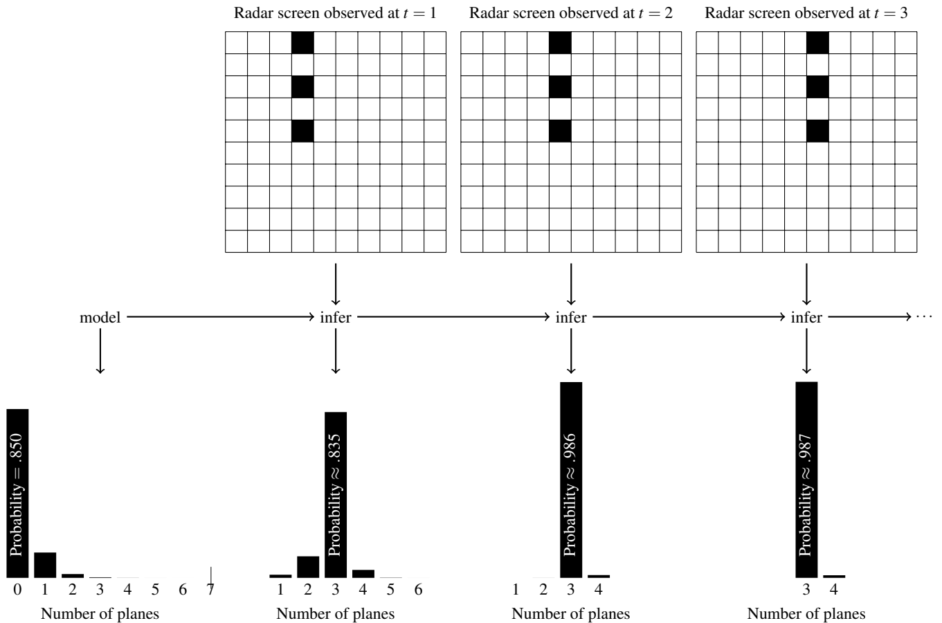
Figure 2. A sample run of aircraft tracking using radar blips. At the top are consecutively observed radar screens. At the bottom are consecutive distributions of the number of planes, first stipulated by the model then gradually computed by our approximate inference.
