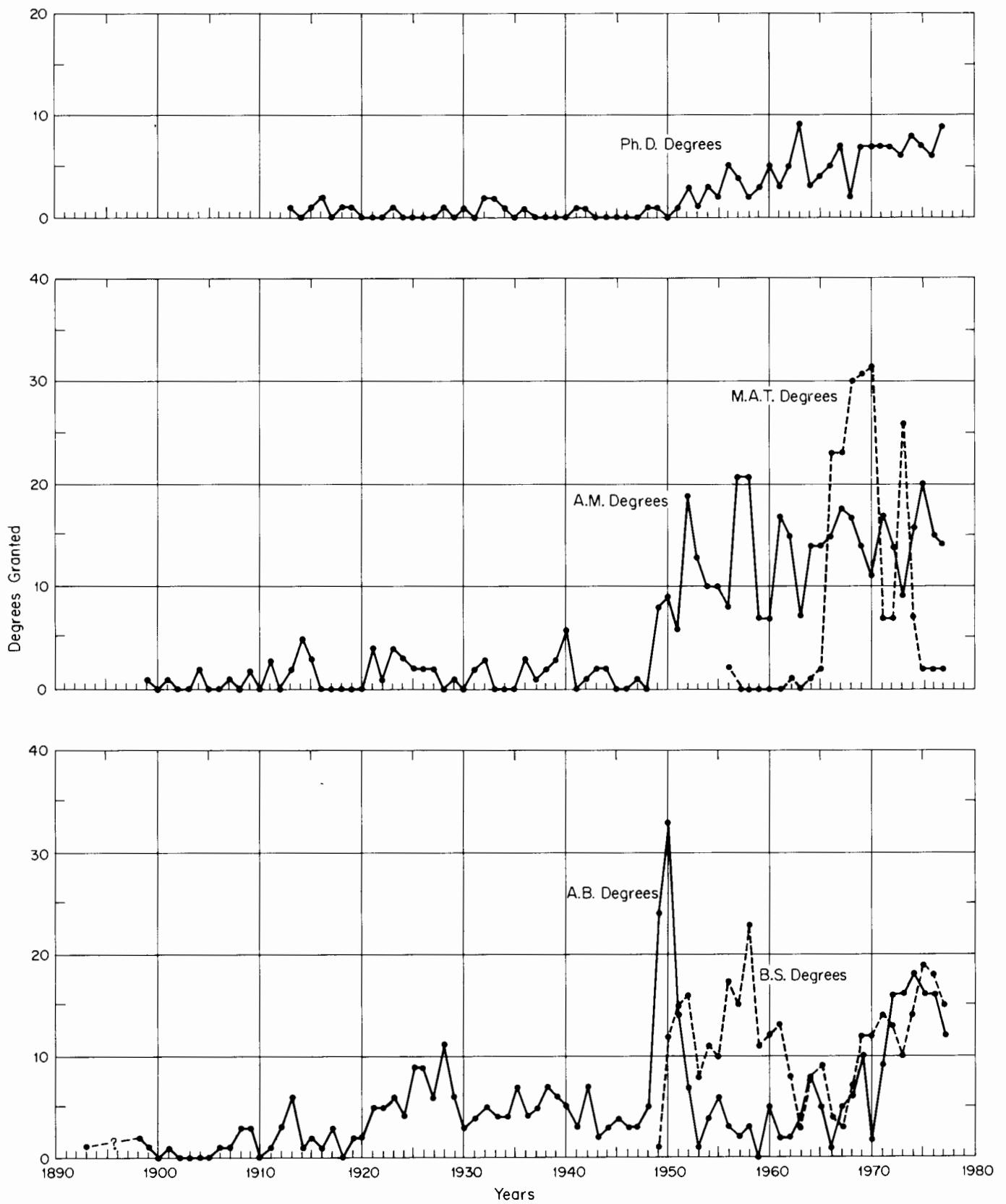
Figure 2—Degrees Granted 1890-1977
