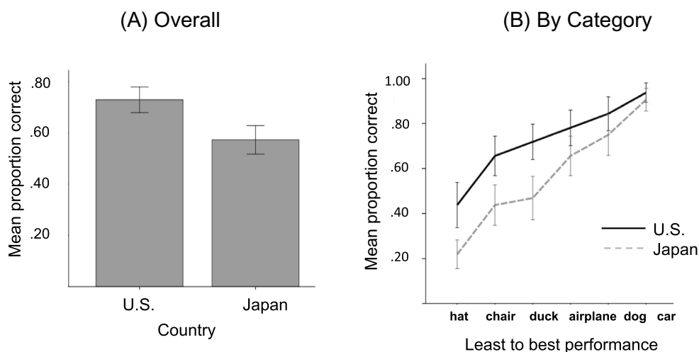
Fig. 2. Results of the Feature task. (A) The bar graph shows mean proportion correct (chance = .16) in recognizing the object from three features for children from the two cultures. (B) The line graph shows proportion correct for the individual categories as a function of culture. The error bars indicates \pm 1 standard error.
